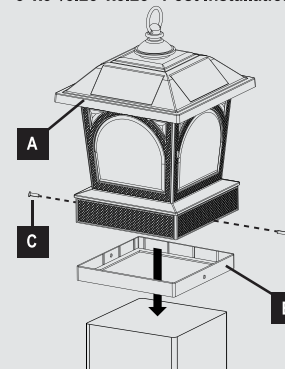
5"x5"/5.25"x5.25" Post Installation
