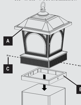
5.5" x 5.5" Post Installation
